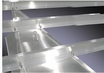
Cross members through-bolted to full length of deck and nosecone
